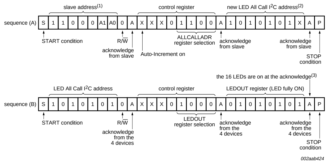
(1) 10-pin version is used for this figure. Four PCA9633DP2s are used and the same sequence (A) (above) is sent to each of them. A[1:0] = 00 to 11. (2) ALLCALL bit in MODE1 register is equal to 1 for this example. (3) OCH bit in MODE2 register is equal to 1 for this example.
